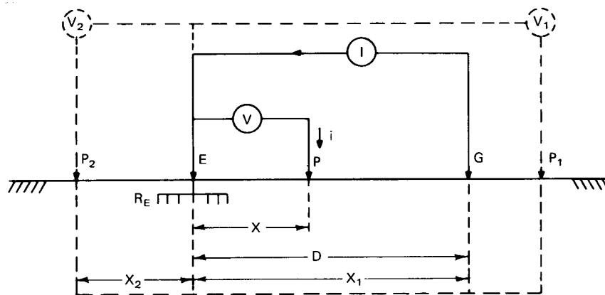
Figure C.1—Fall-of-Potential Method
