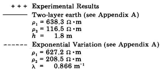
Figure 5—Example of an Earth Resistivity Interpretation
