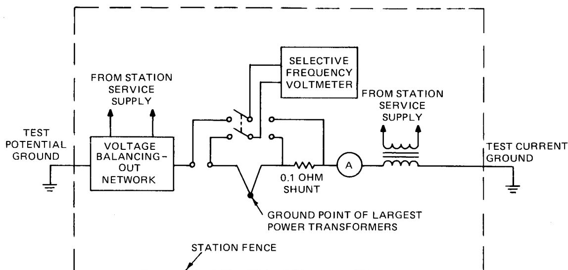
Figure 17—Selective-Frequency Voltmeter-Ammeter Circuit
