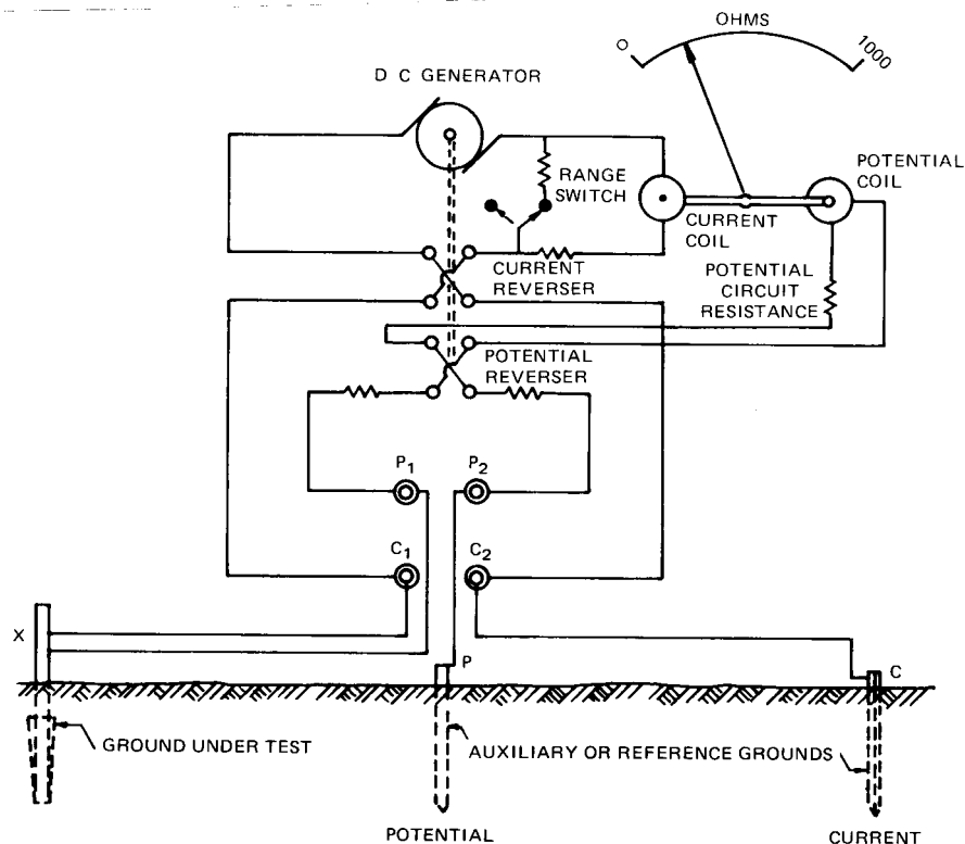
Figure 14—Ratio Ohmmeter
