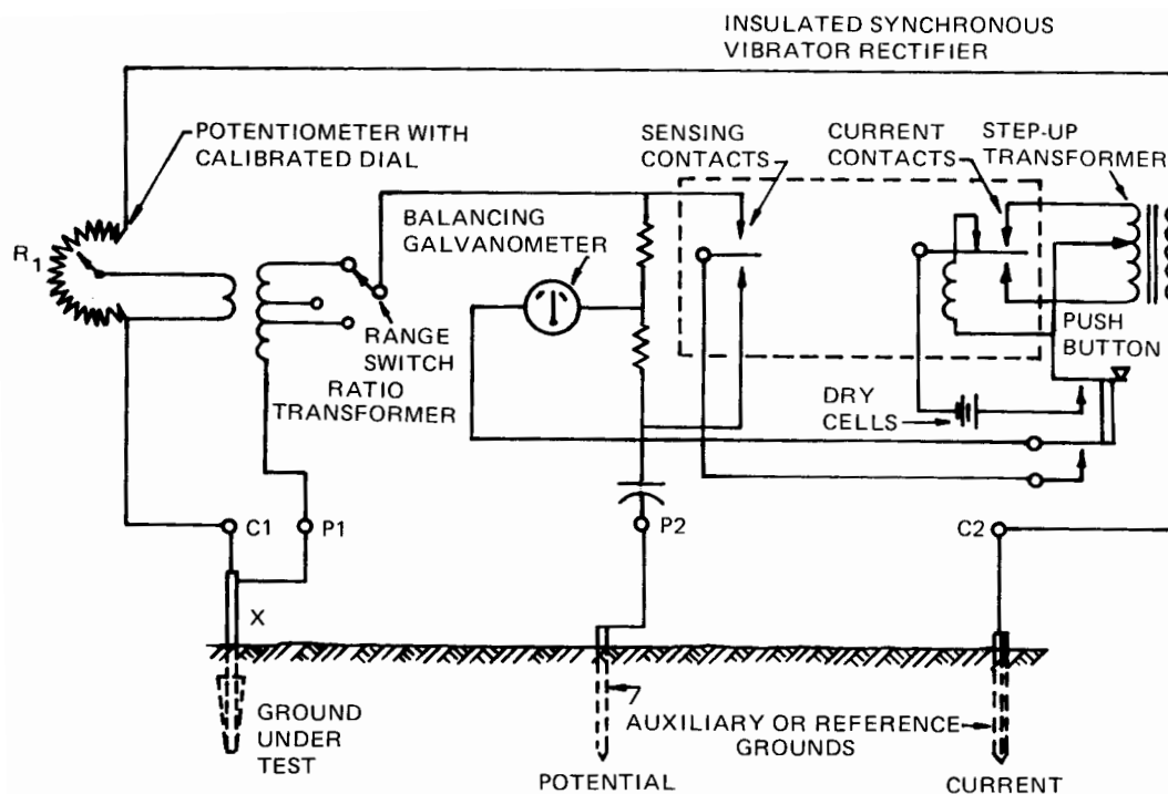
Figure 16—Single-Balance Transformer
