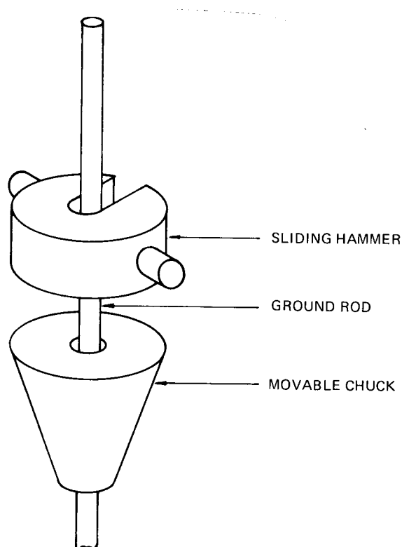
Figure 20—Chuck and sliding Hammer
