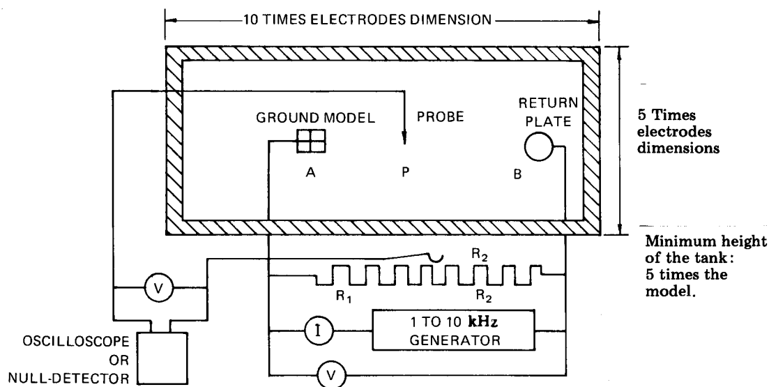
Figure 13—Electrolytic Tank
