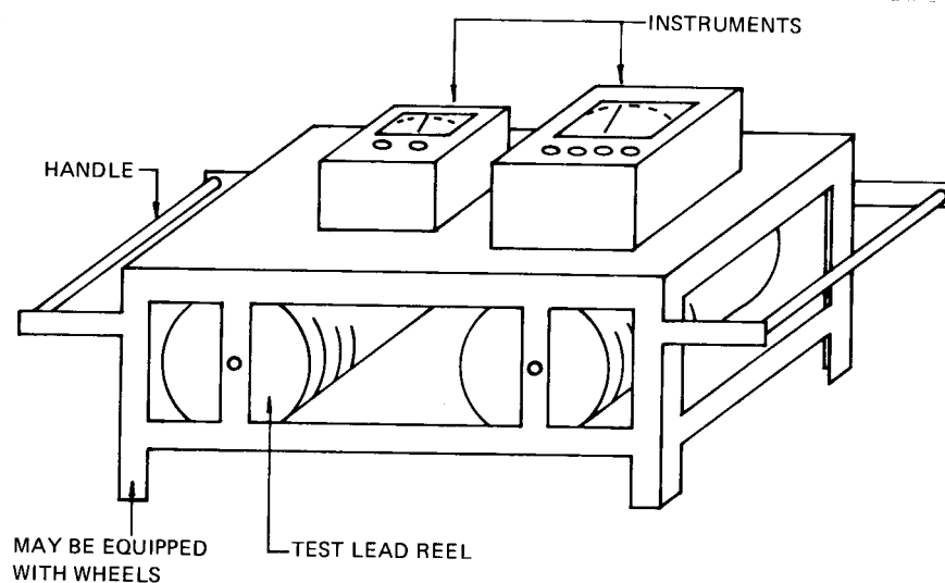
Figure 21—Test Table
